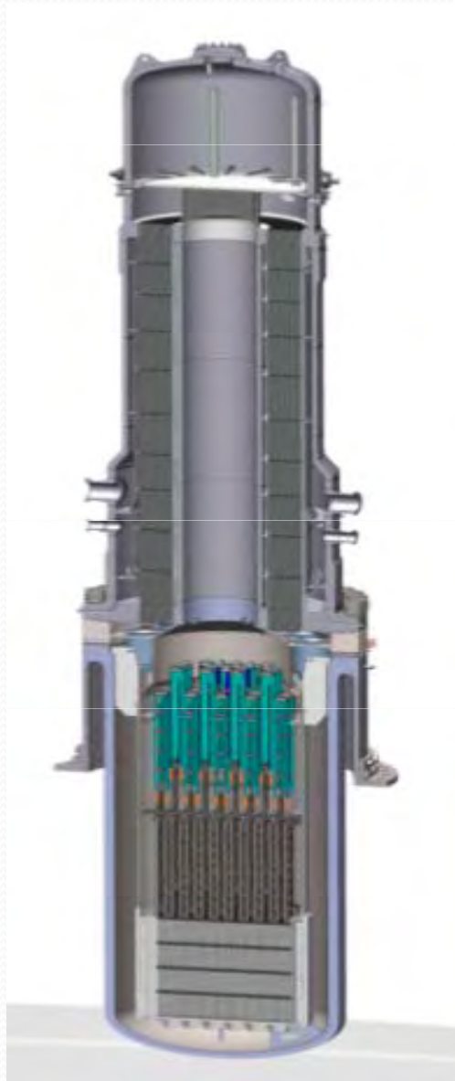
mPower – B&W
