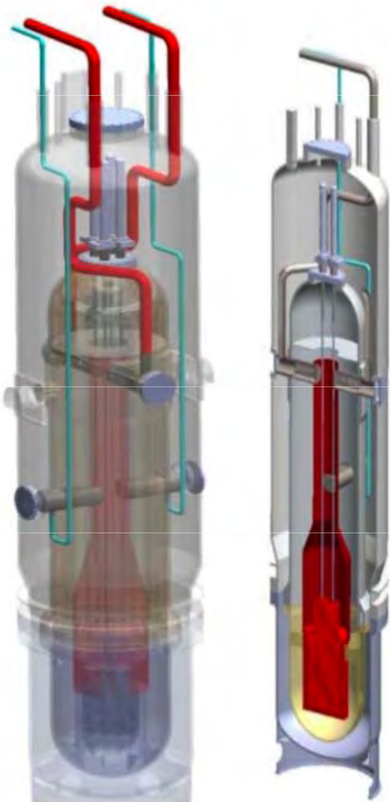
NuScale PWR
